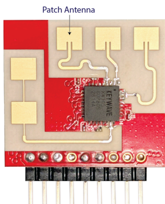
Module Front side (antenna facing forward)
